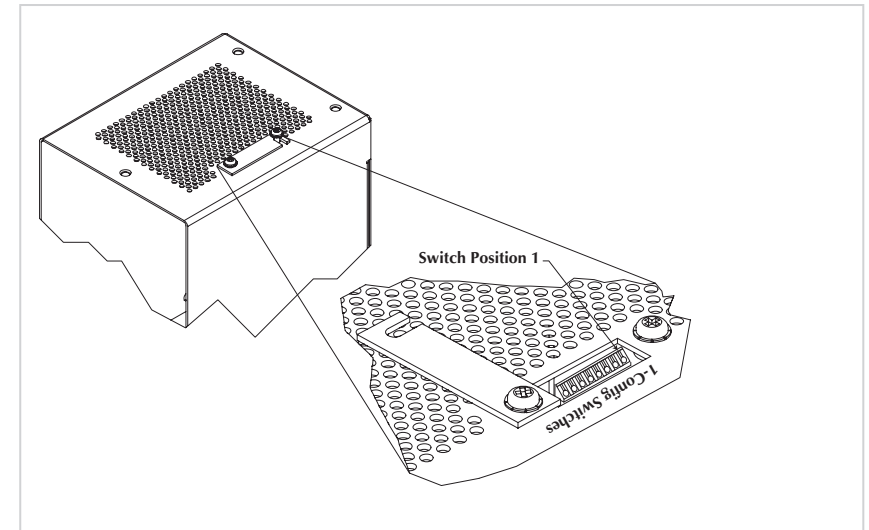
Figure 4: Enclosure Top View Configuration Switches
